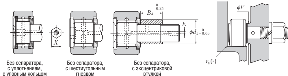
FCRS
