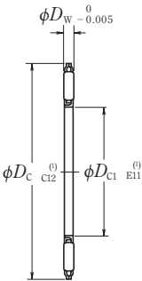
FNTA
